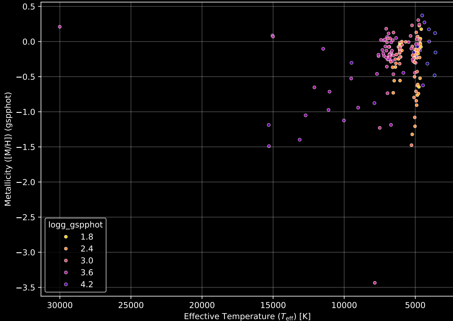
APOGEE DR17 Field: [158+00] Stellar Population Parameters (n= 170)
