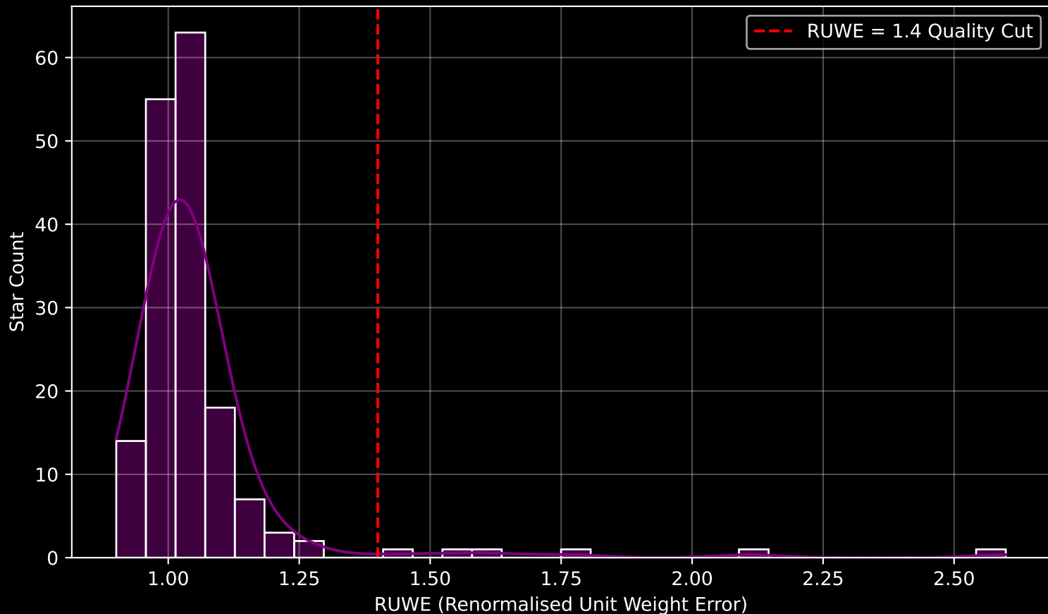
GAPOGEE DR17 Field [158+00] RUWE Distribution (n= 168)
