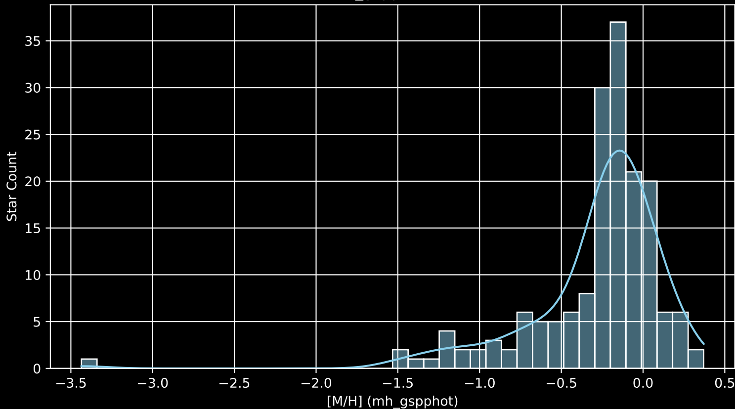
APOGEE DR17 Field: [158+00 [M/H] (mh_gspphot) (n= 170)
