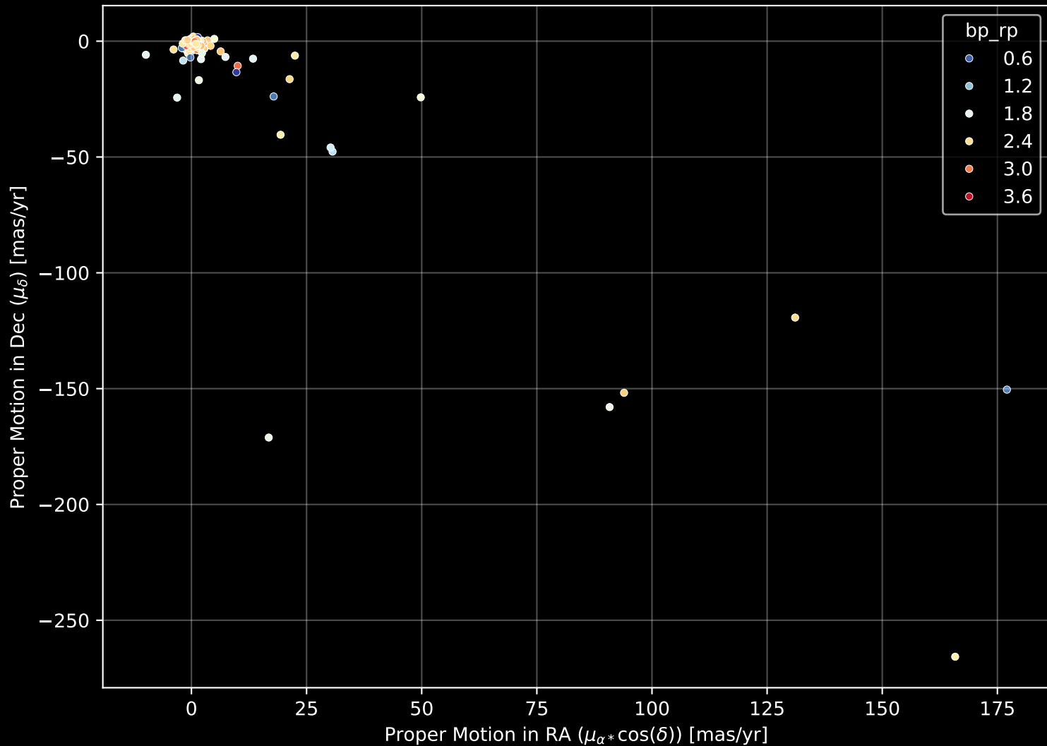
APOGEE DR17 Field: [158+00] Proper Motion Diagram (n= 170)
