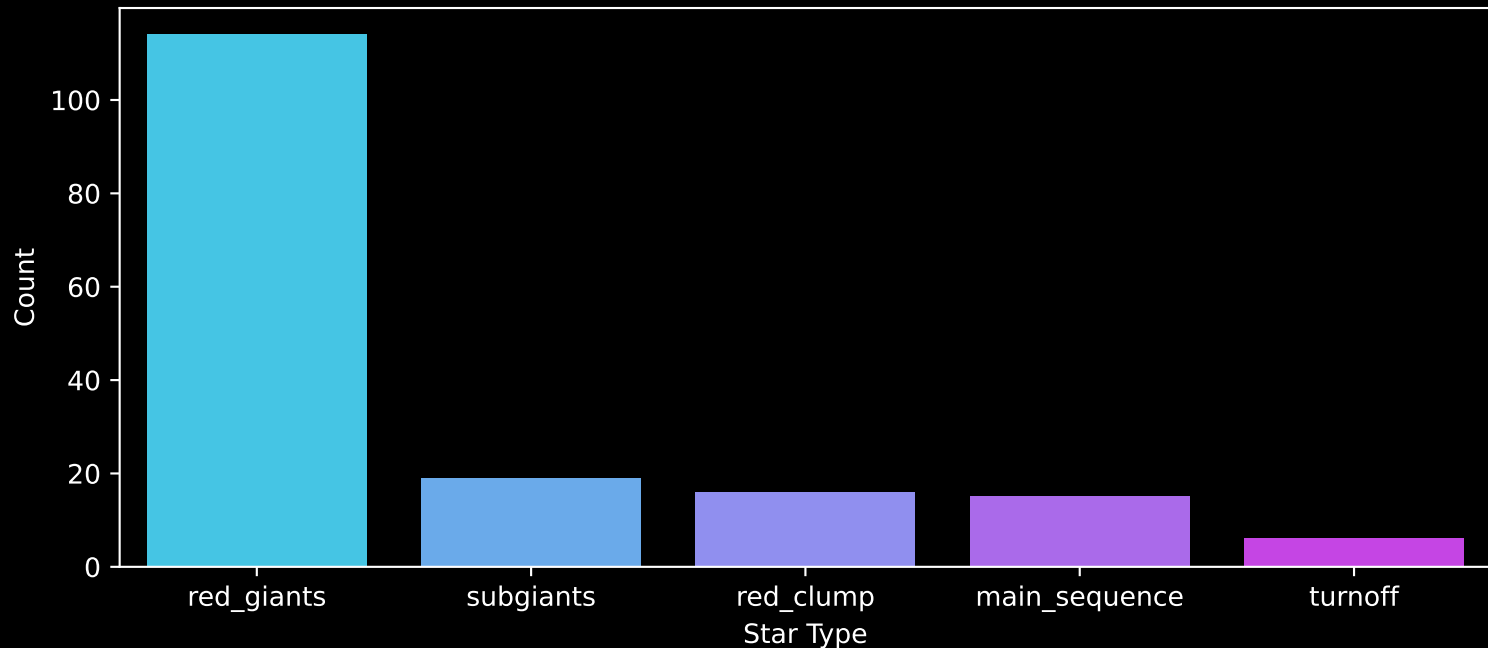
APOGEE DR17 Field: [158+00] Count plot of Star Type
