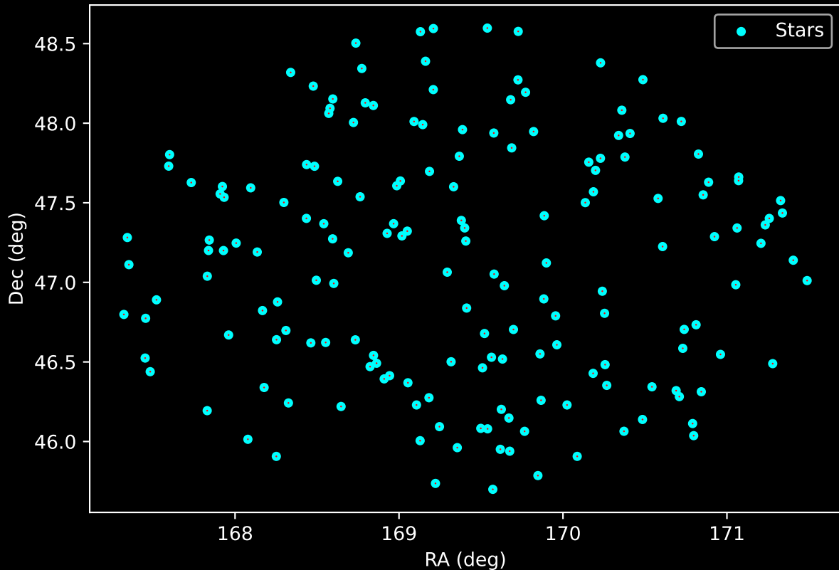
APOGEE DR17 Field: [158+00] Proper Motion Vectors for Gaia Star Field (n= 170)
