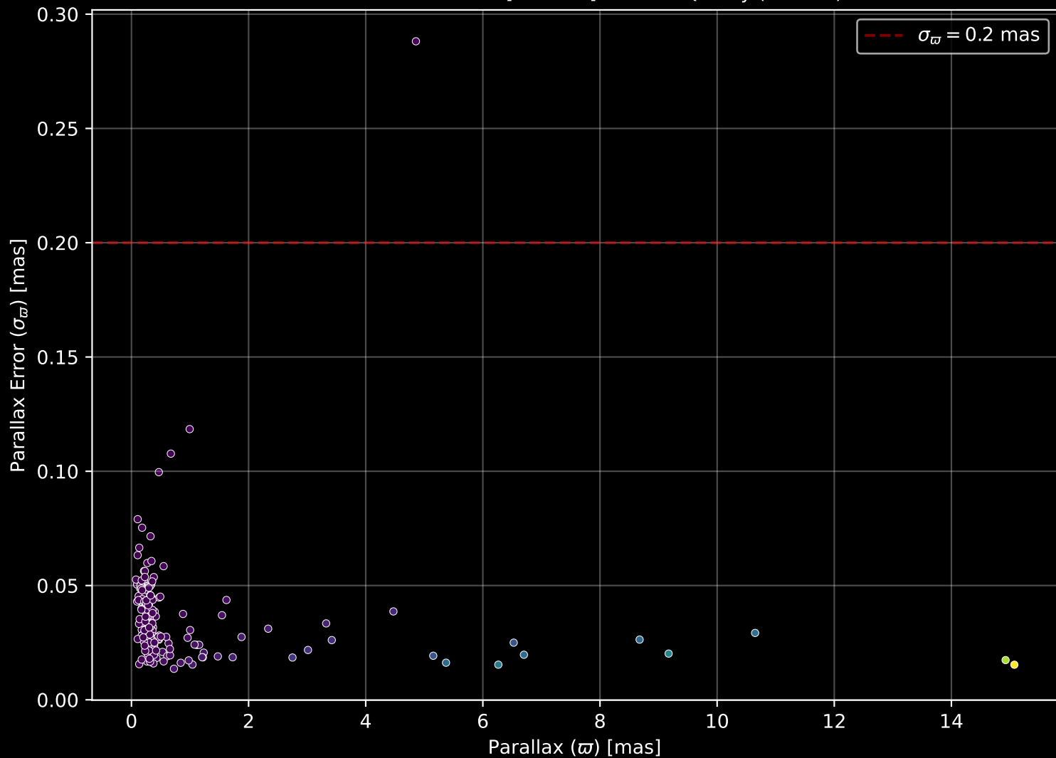
APOGEE DR17 Field: [158+00] Parallax Quality (n= 170)
